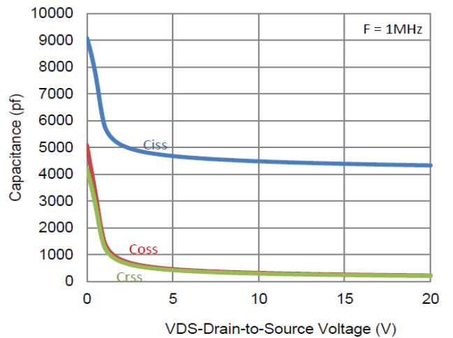
6. Capacitance
