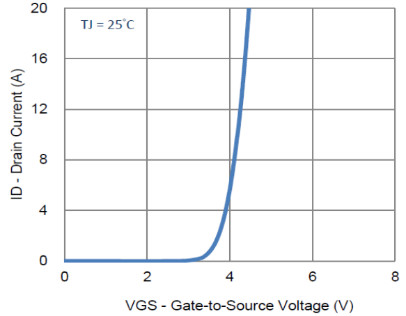
2. Transfer Characteristics
